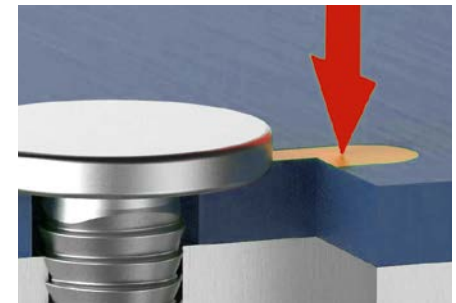
Ground connection PCB / bolt possible
