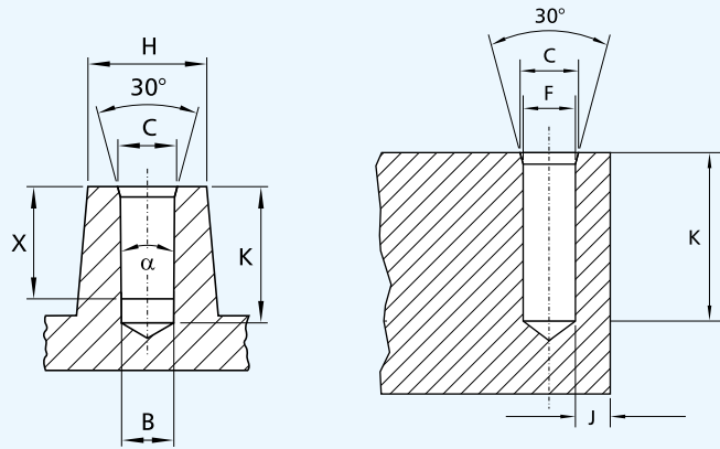
Core hole recommendation for cast holes. Max. draft angle \alpha = 1^\circ
